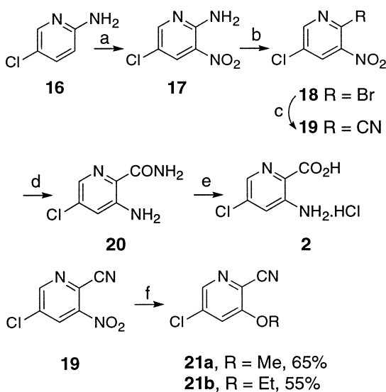
Scheme 3. (a) HNO 3 /H 2 SO 4 /60 °C, 67%; (b) NaNO 2 /HBr/Br 2 , 65%; (c) CuCN/185 °C, 92%; (d) Raney Ni/H 2 /95% EtOH, 95%; (e) concd HCl, reflux, 85%; (f) ROH/10% NaOH/rt.
